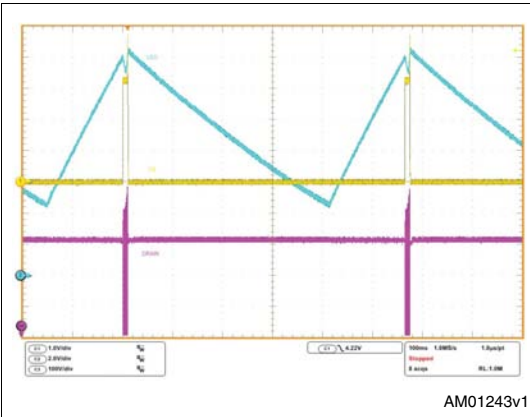
Figure 13. V_{IN} = 115\text{ V}_{AC} - 60 Hz short-circuit operation
