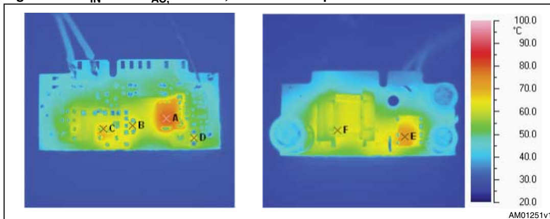
Figure 22. V_{IN} = 230\text{ V}_{AC} , full load, bottom and top sides
